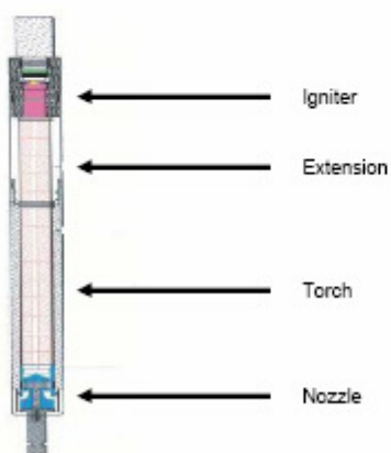
Radial Cutting Torch Schematic
