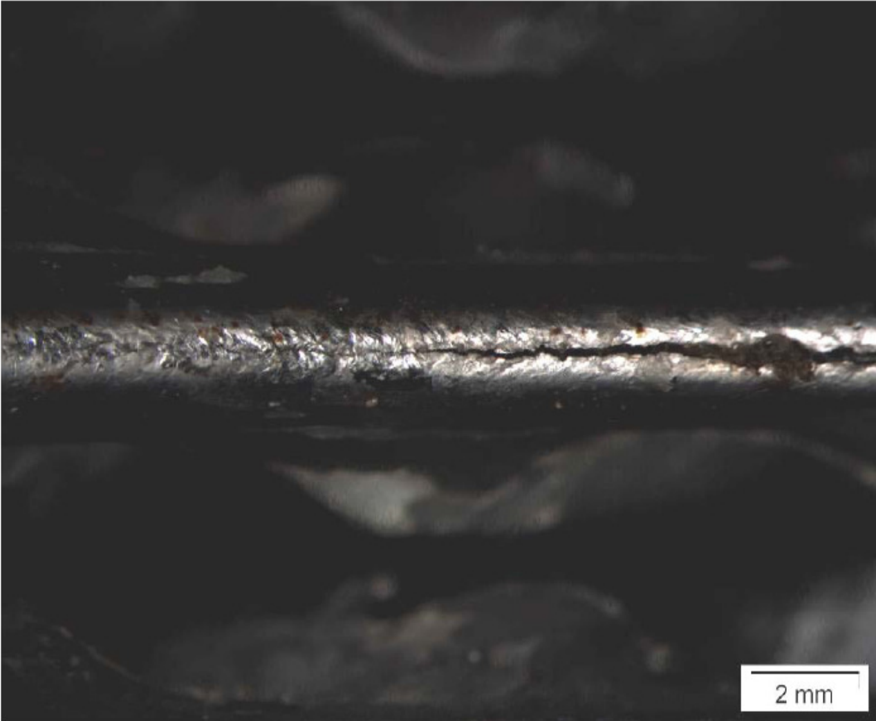
Magnified view of cracked weld plate:
